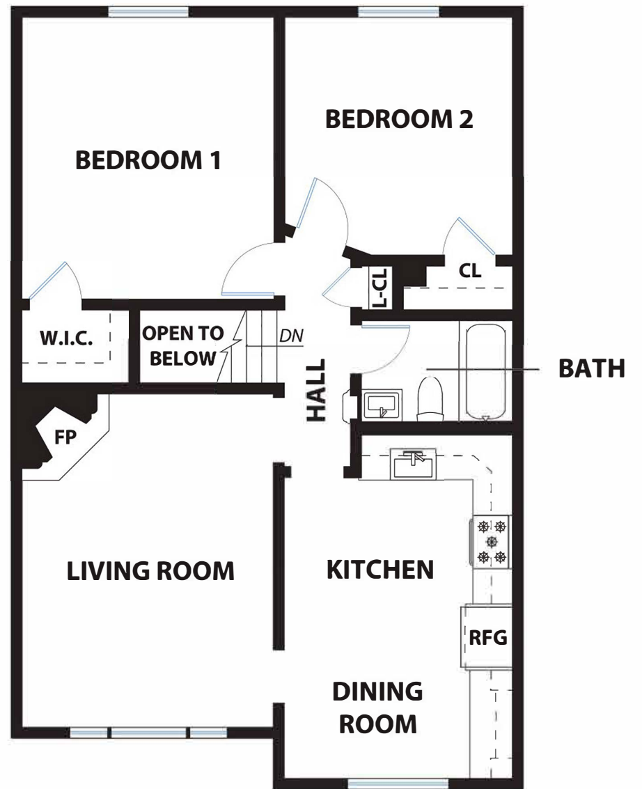
MAIN LEVEL
